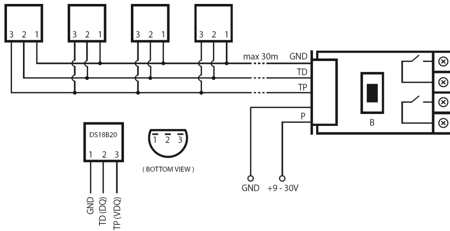
Diagram 4 – Connection to DS18B20 sensors
