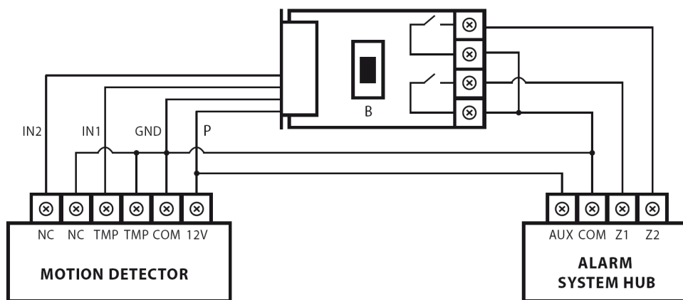
Diagram 2 – Connection to a regular alarm line
