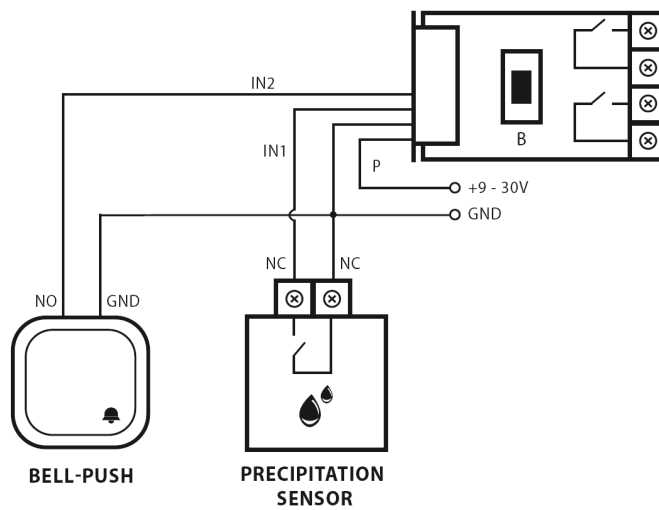
Diagram 5 – example connection to a precipitation sensor
