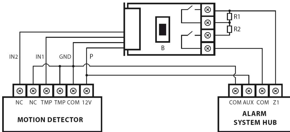
Diagram 3 – Connection to a parametric alarm line
